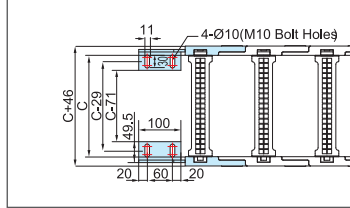
Moving End
