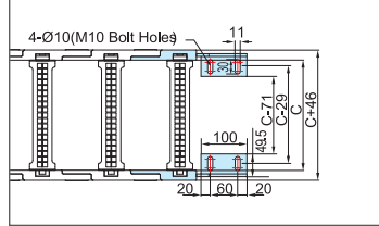
Fixing End
